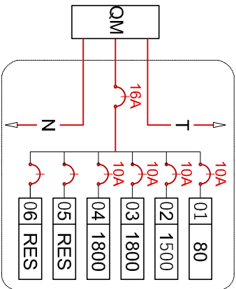
DIAGRAMA UNIFILAR
