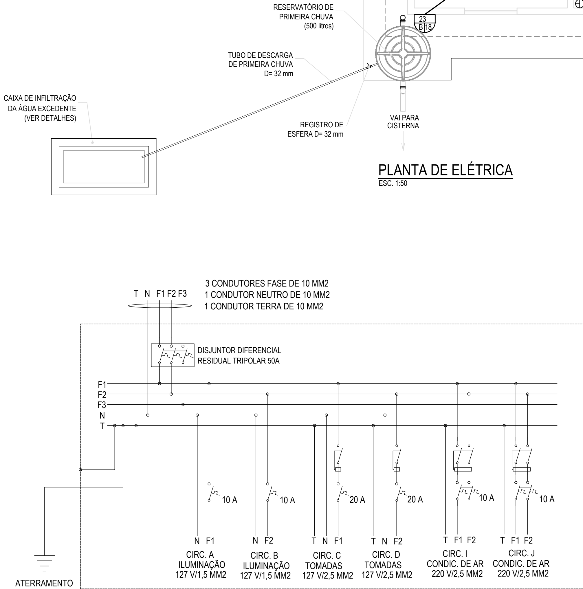
DIAGRAMA UNIFILAR
