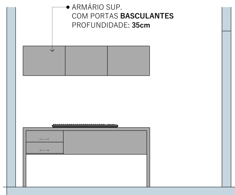
VISTA FRONTAL
