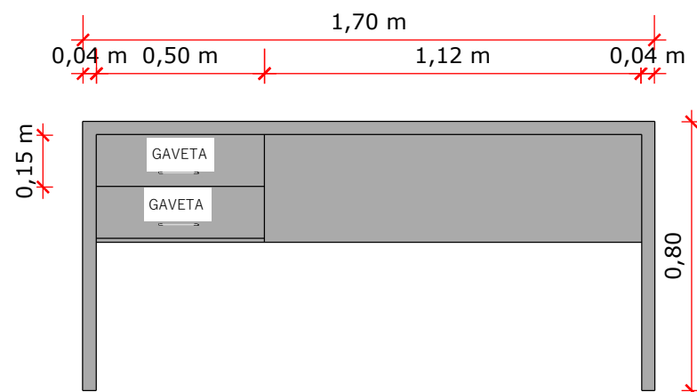
MESA - VISTA FRONTAL
