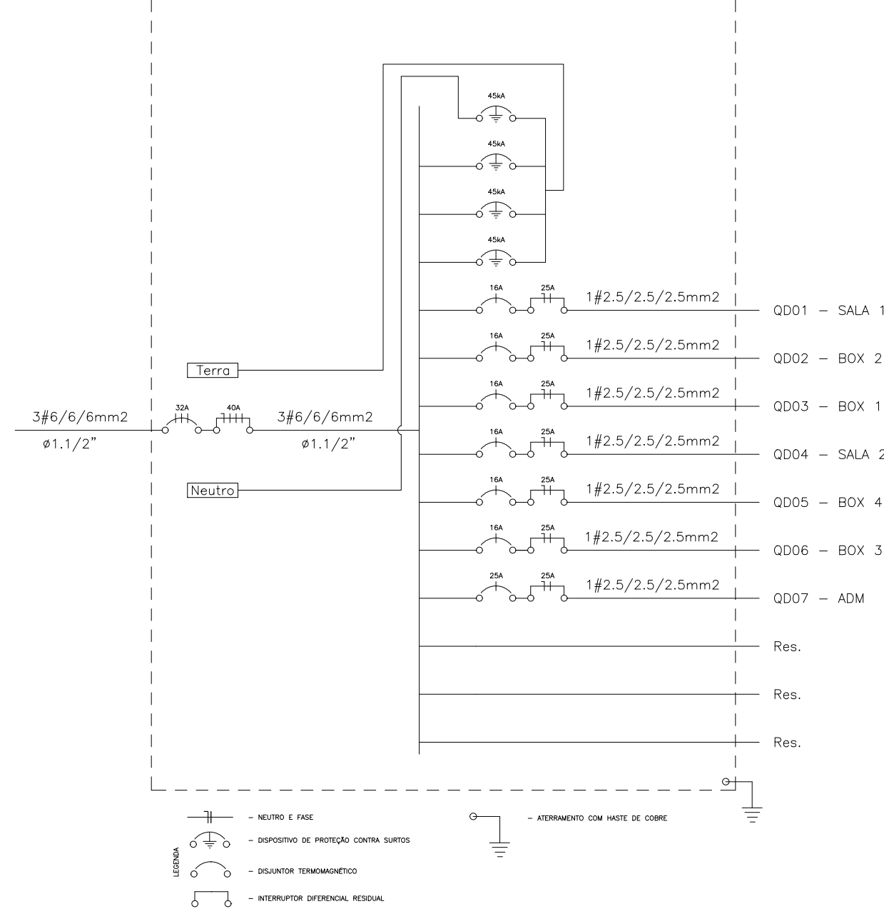
03 DIAGRAMA UNIFILAR
